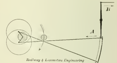
FIG. 12. "CROSSED" RODS WITH ROCKER ARM.
